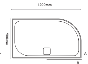
Offset Quadrant Tray
