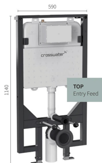
Ultra Slim 1.14m Toilet Frame
