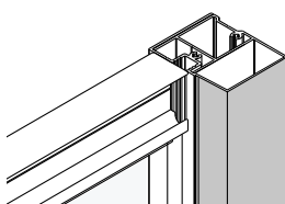
With cover strip - conceals all fixings - cover strips can be cut down to 1800mm for loft height enclosures.
