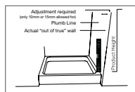
Diagram 3 Out of True Wall
