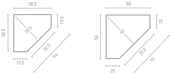
Tyne Unit Sizes
