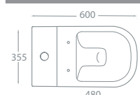
600mm Projection
